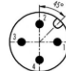
Female insert M12
