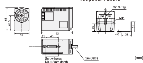
Amplifier Fixture
